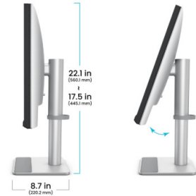
115mm Height Adjustment | Tilt -5~20°
