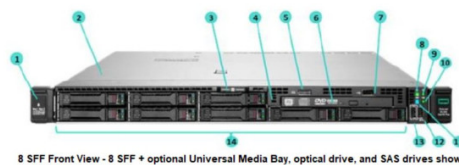
8 SFF Front View - 8 SFF + optional Universal Media Bay, optical drive, and SAS drives shown
